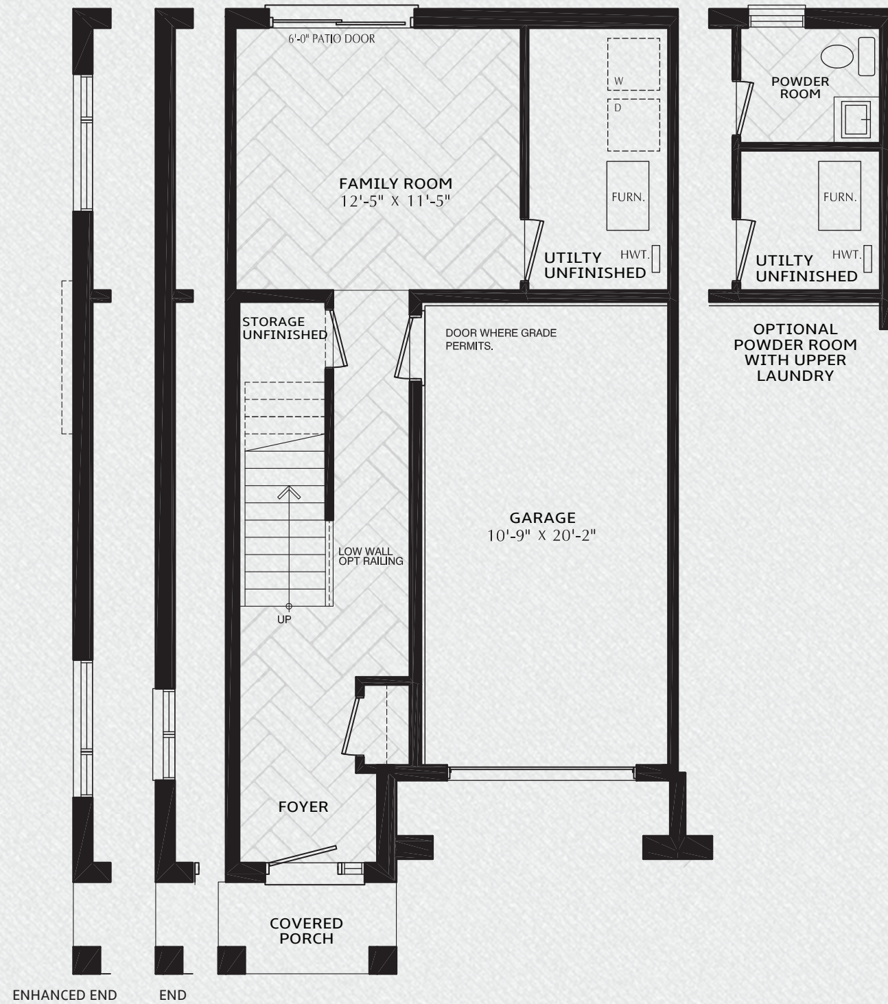
GROUND FLOOR
