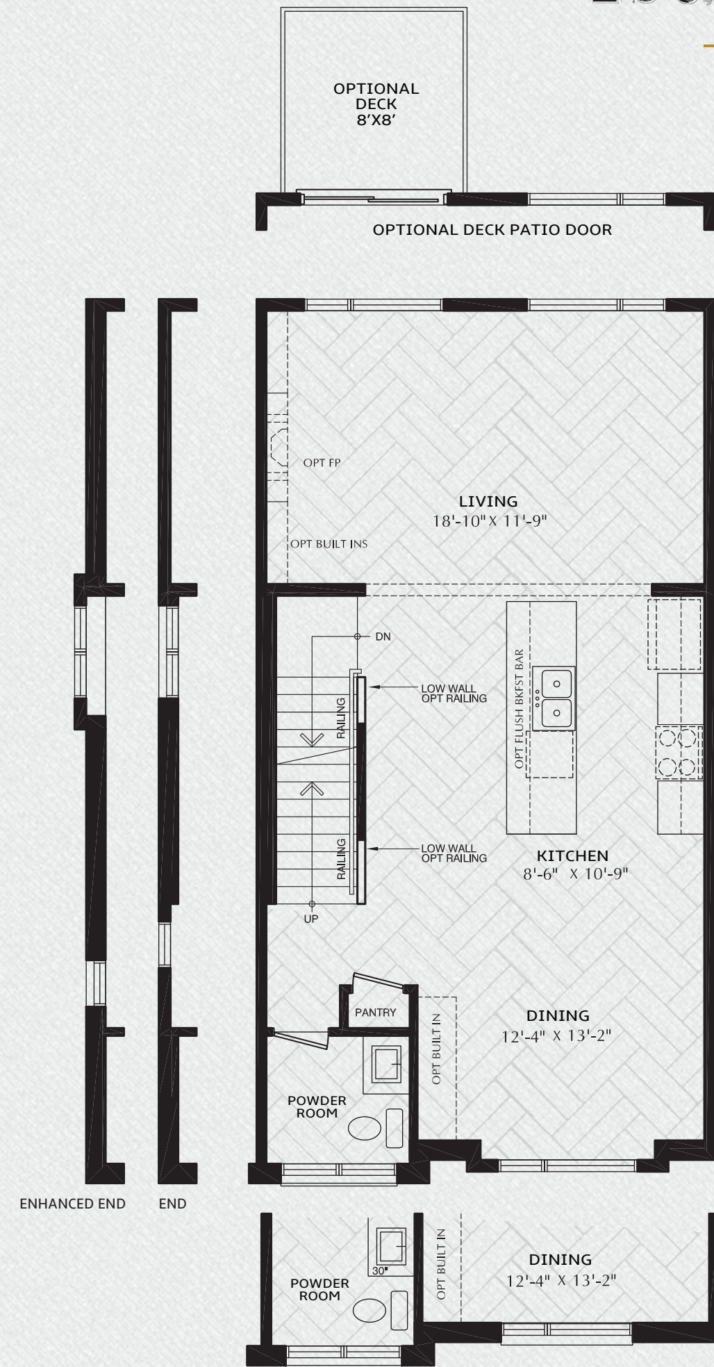
SECOND FLOOR
