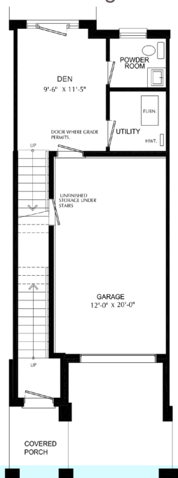
Ground Floor 9' Ceiling
