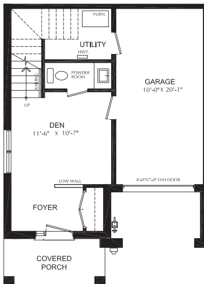
Main Floor 9' Ceiling
